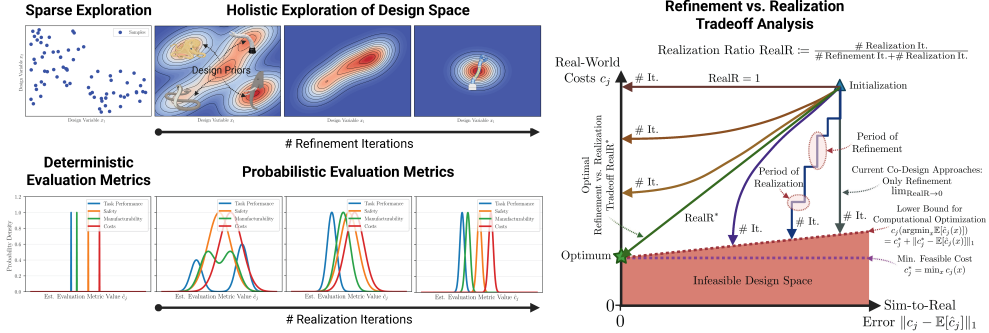
Fig. 4 Refinement vs. Realization. Top Left: This panel shows how refinement affects the design sampling distribution \vartheta(x) . Unlike (most) conventional co-design methods that sparsely explore the design space, we condition \vartheta(x) on design priors (e.g., biological inspiration and existing soft robot designs) and iteratively update it via the co-design optimizer until the optimum is reached. Bottom Left: Here, we demonstrate how iterative realization refines probabilistic evaluation metrics. Rather than using deterministic metrics that ignore inherent simulation uncertainty, we define a probabilistic distribution \hat{m}_j(\hat{c}_j, x) for each metric, with purposeful prototyping reducing the uncertainty over iterations. Right: This panel examines the tradeoff between refinement and realization. We define the realization ratio \text{RealR} as the fraction of realization iterations relative to the total iterations and the sim-to-real error as \|c_j - \mathbb{E}[\hat{c}_j]\| . We then plot the evolution of real-world cost c_j versus sim-to-real error as iterations increase for a fixed \text{RealR} : when \lim \text{RealR} \rightarrow 0 , designs are optimized computationally with realization occurring only at the end, while \text{RealR} = 1 means only the confidence in the evaluation metrics is increased. The optimal ratio \text{RealR}^* efficiently minimizes the real-world cost to its optimum \min_x c_j(x) via refinement and reduces the sim-to-real error to zero by updating \hat{m}_j(\hat{c}_j, x) via realization.
