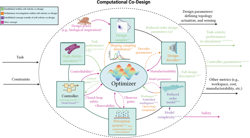
Fig. 3 A Framework for Efficient Computational Co-Design of Soft Robots. We sample reduced-order design parameters x from an initial distribution that can include design priors from biological inspiration [24, 96, 99], known mechanisms, or existing soft robot designs. This design space—either learned or explicitly defined by physical or geometric values (i.e., size optimization)—is translated by a design decoder into a detailed robot body description (such as a 3D mesh with sensor and actuator placements) that provides immediate manufacturability feedback. A reduced-order model is then derived [46, 48, 49, 60] or learned to efficiently assess workspace, open-loop compliance, and embodied intelligence [69, 100, 101], offering inexpensive feedback to the optimizer. Similarly, perception and control systems can be developed using this model (via model-based control [47], MPC [46], or differentiable physics [23, 35]), while observability and controllability are evaluated without costly simulations. Finally, closed-loop simulations (low-fidelity using the reduced-order model or high-fidelity FEM-based [91]) assess integrated performance metrics, which in turn optimize the sampling distribution, decoder, and all relevant system parameters. References in graphic: (1): [33], (2): [25], (3): [35], (4): [32], (5): [44], (6): [55], (7): [54], (8): [34], (9): [38], (10): [58], (11): [60], (12): [49], (13): [102], (14): [46], (15): [26], (16): [30], (17): [51], (18): [103], (19): [69], (20): [100], (21): [101], (22) [23], (23): [47].
